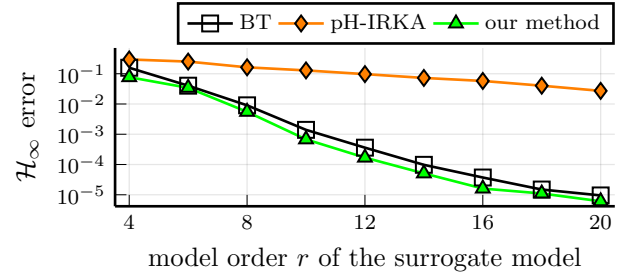
Fig. 2. \mathcal{H}_\infty error comparison for different MOR methods
